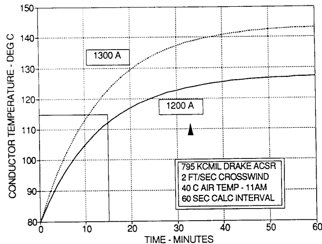
Figure 2—Conductor temperature vs. time curves
