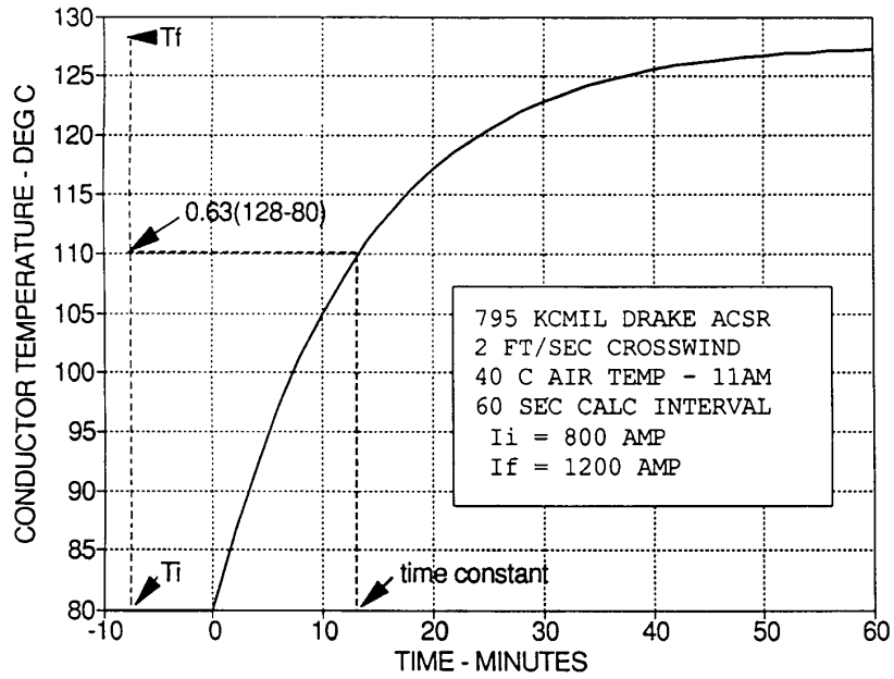
Figure F1—Conductor temperature vs. time curve
